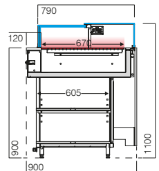
VMINTA B - VDB UV tampo aquecido heated deck plaque chauffante tampo caliente
