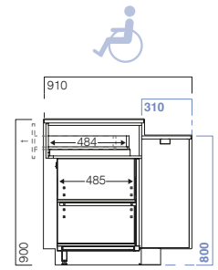
VMINPMR B caixa PMR PMR support counter caisse PMR caja PMR
