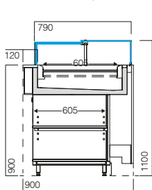
VMINNT B - VDB UV neutra dry ambient neutre neutra
