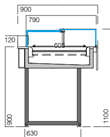
VMINNT P - VDB UV neutra dry ambient neutre neutra
