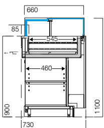
VMINSPOS - VDB UV padaria bakery boulangerie panaderia
