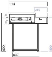
VMINPMR P caixa PMR PMR support counter caisse PMR caja PMR
