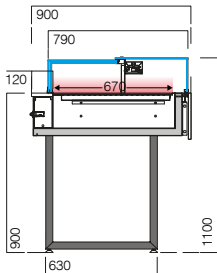
VMINTA P - VDB UV tampo aquecido heated deck plaque chauffante tampo caliente
