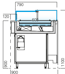
VMIND - VDB UV 3M2/3S dupla temperatura dual-temperature dual-temperature dual-temperature
