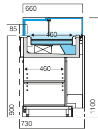
VMINSD - VDB UV 3M2/3S dupla temperatura dual-temperature dual-temperature dual-temperature
